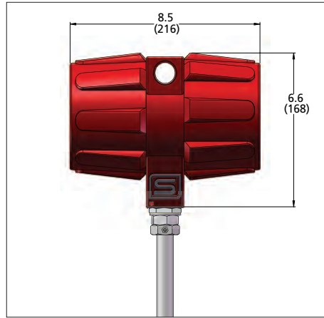
P2-DD Flange Fitting—Side View
